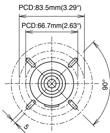
Mounting Base
